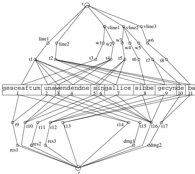
Figure 2: The KyGODDAG data structure for the encodings in Figure 1
